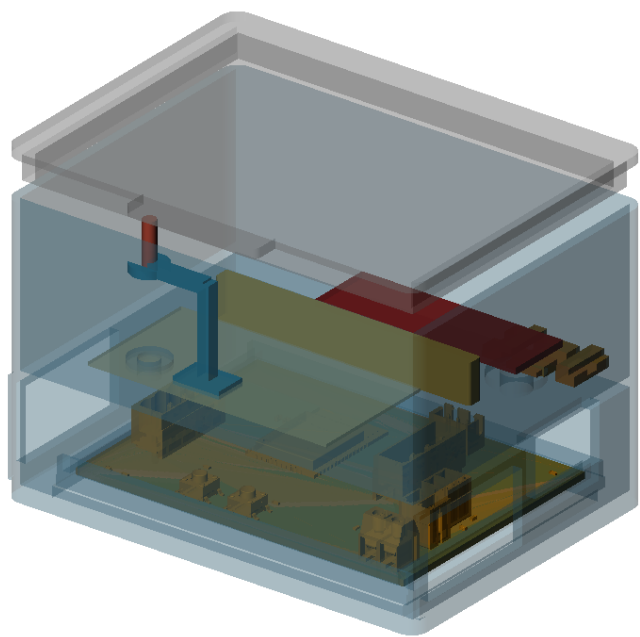
Figure 4.3 – Three-dimensional enclosure layout with PCB reference
