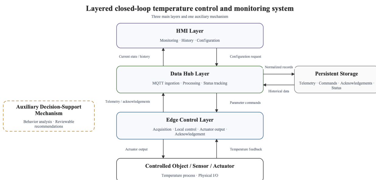
Figure 3.1 – General architecture of the developed system
