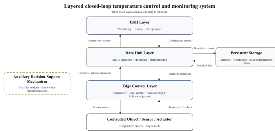
Figure 3.1 – General architecture of the developed system
