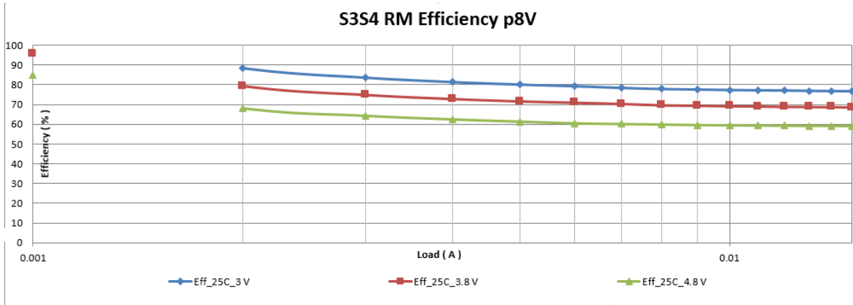
Figure 3-3 S3-S4 efficiency, retention mode
