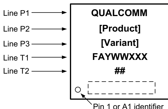
Figure 4-2 PM6225/PM6375 device marking (top view, not to scale)
