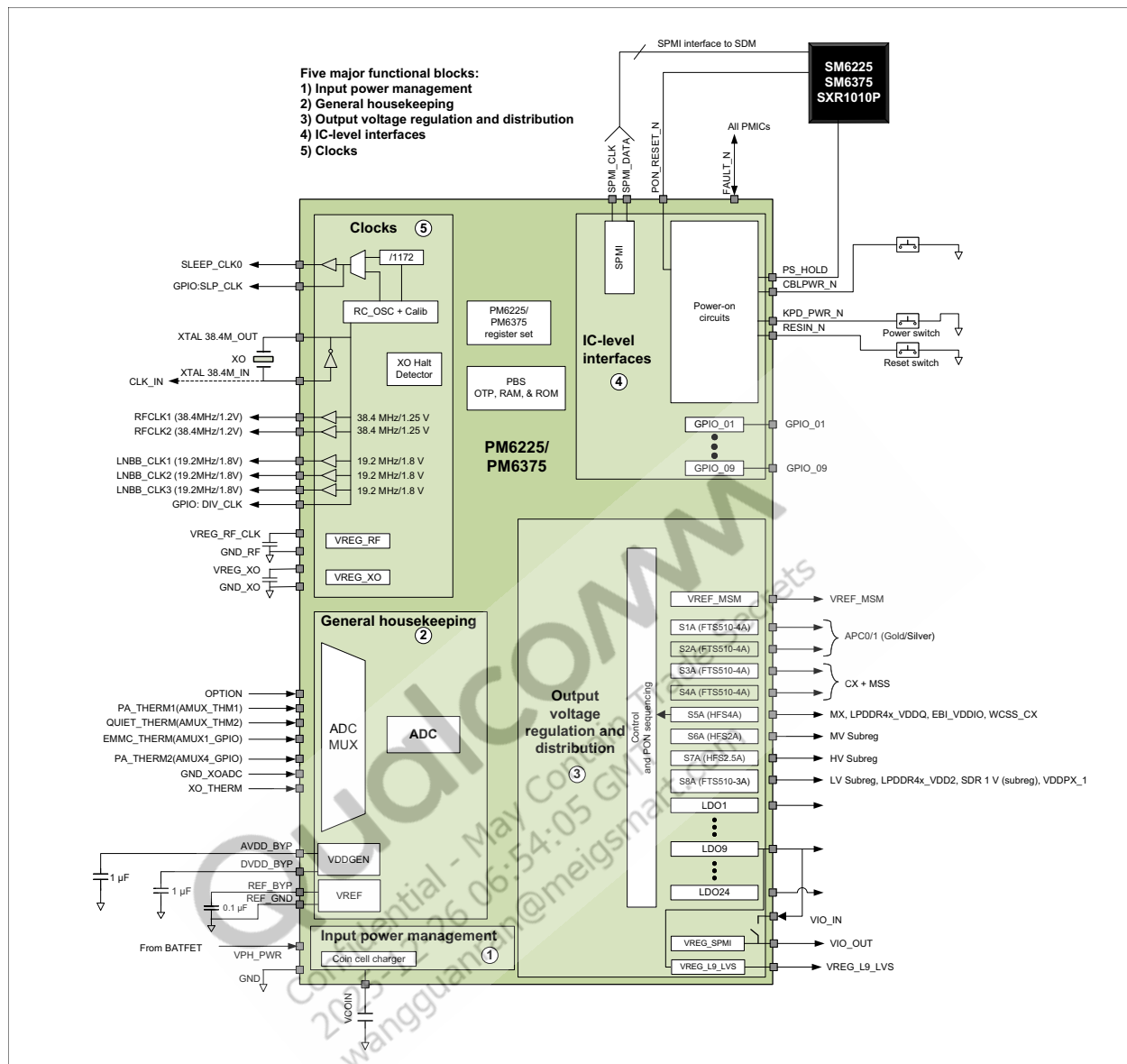
Figure 1-1 PM6225/PM6375 functional block diagram and example application
