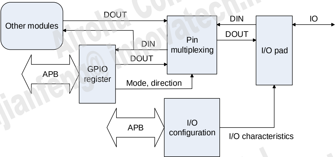
Figure 6.1-2. GPIO block diagram
