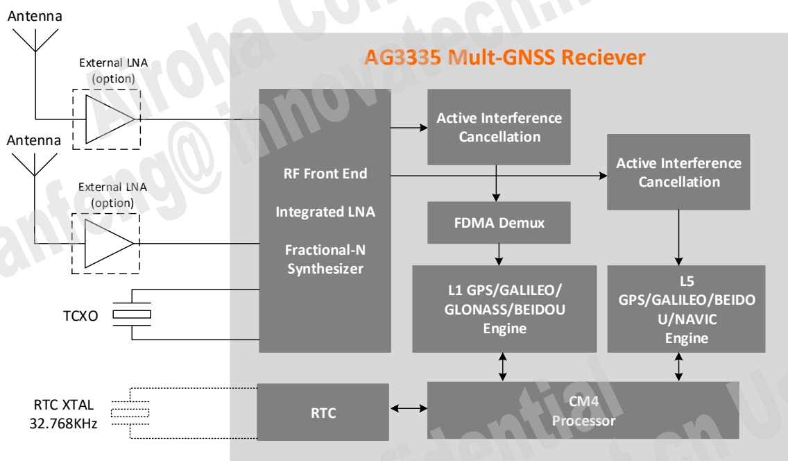
Figure 3.4-1. AG3335M Multi-GNSS receiver block diagram
