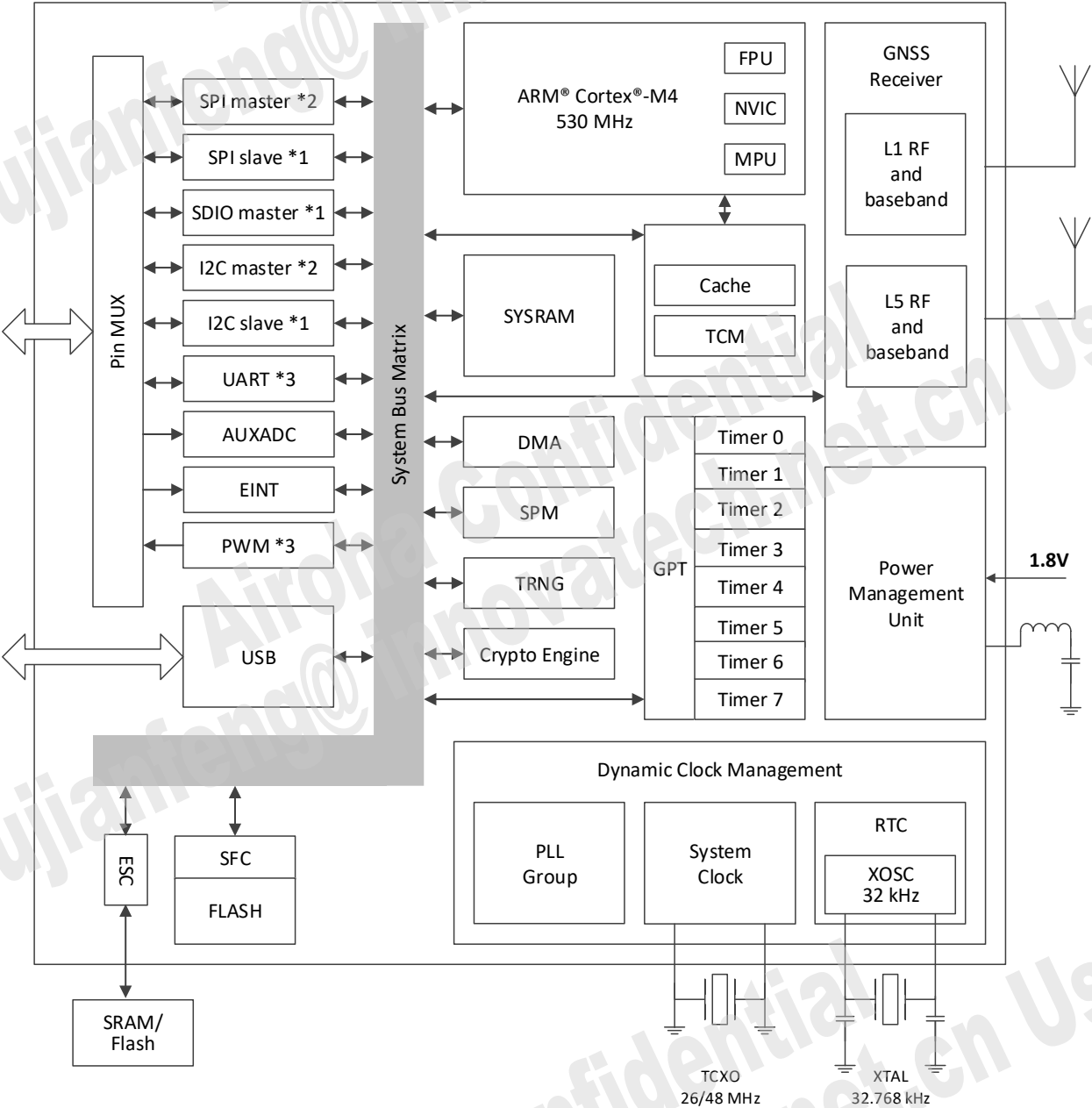
Figure 1.2-1. AG3335M chip architecture
