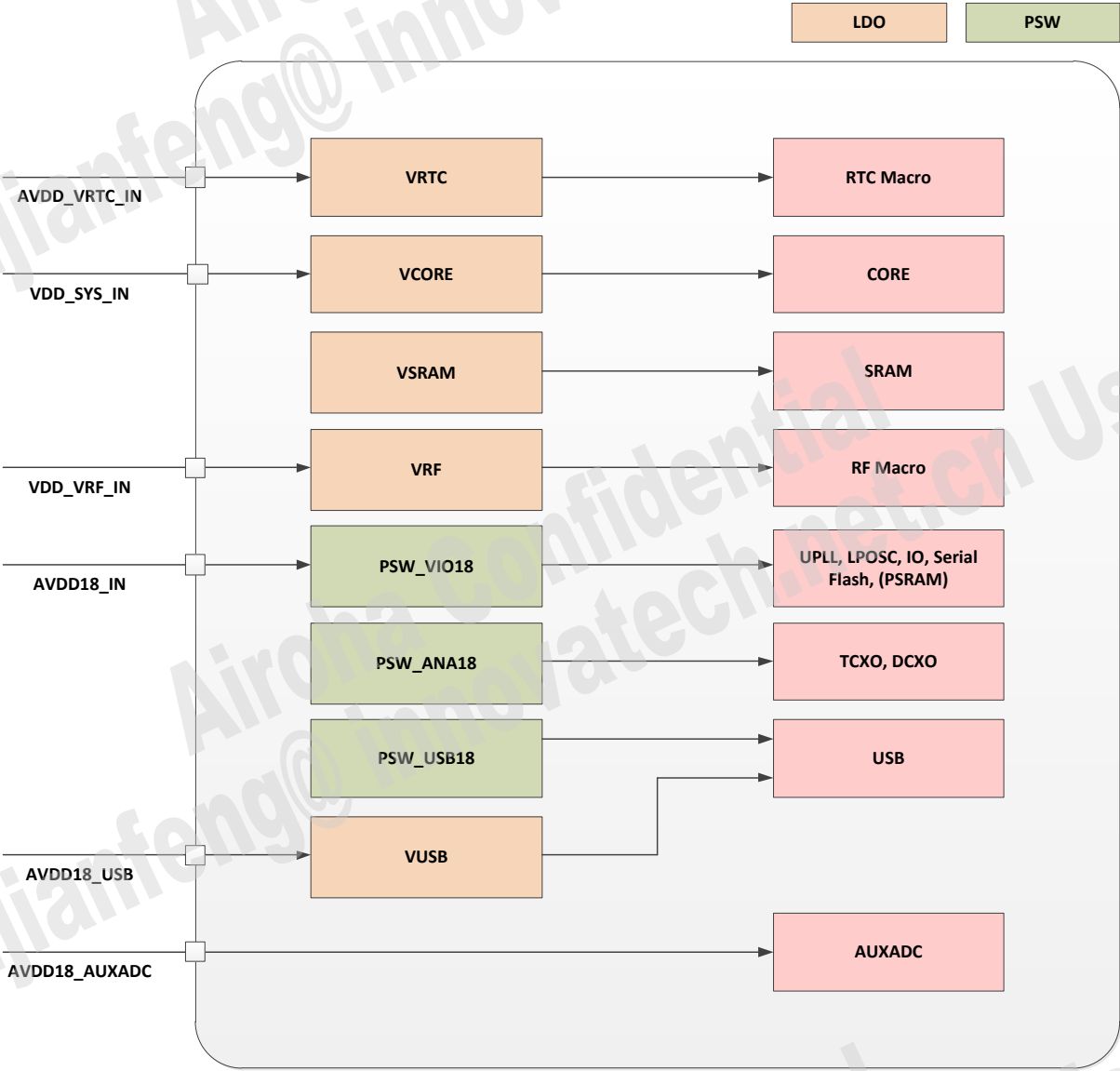
Figure 5.3-1. AG3335M power grid
