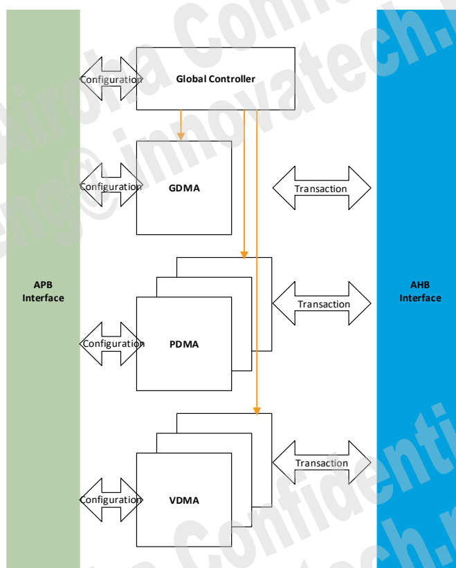
Figure 2.4-2. DMA block diagram
