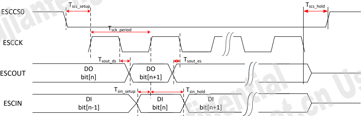
Figure 7.4-9 ESC interface timing
