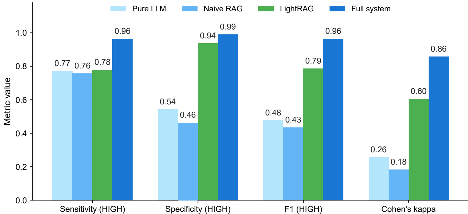
L1 literature-consensus benchmark: 4-method comparison (5 seeds)
