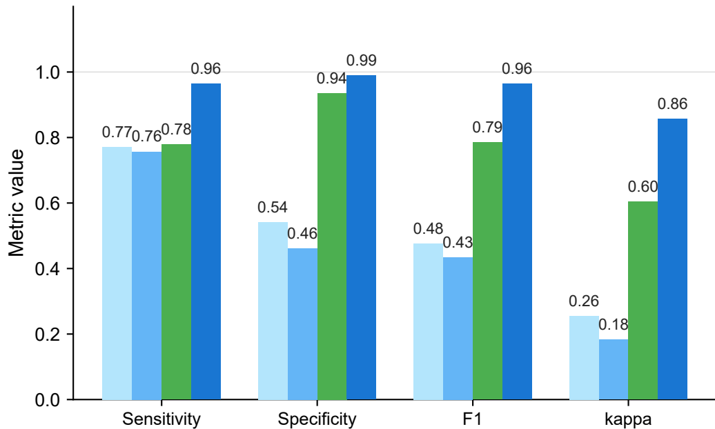
(a) 10-token, single call
