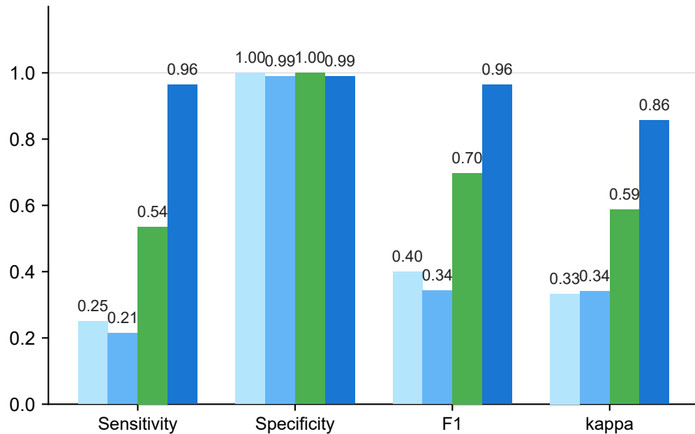
(b) 3000-token, reasoning model, majority of 5
