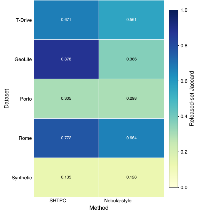
Fig. 6. Fixed-configuration released-set Jaccard at N=1000 and T=10 , averaged over seeds 101, 202, and 303. Both methods use \varepsilon=5.0 . SHTPC uses post-admission release threshold \tau=2.0 . Table VI reports standard deviations, absolute deltas, FRR, and MRR.
