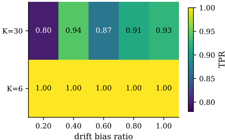
ADWC TPR on gradual-drift attack
