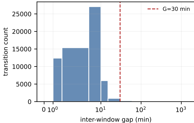
T-Drive
