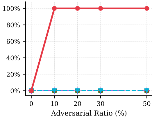
Attack Detection (TPR)
