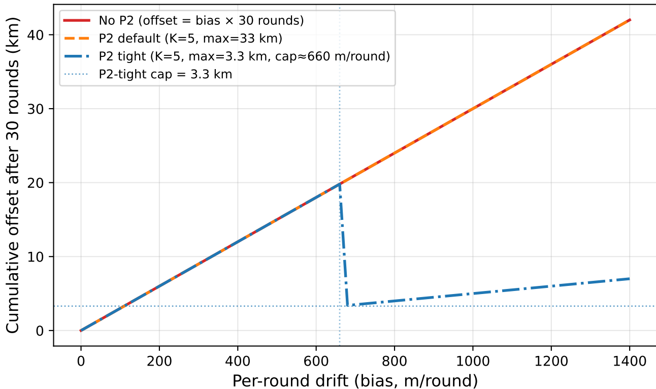
A3 Gradual Drift: Offset vs. Bias Under Different P2 Configs
