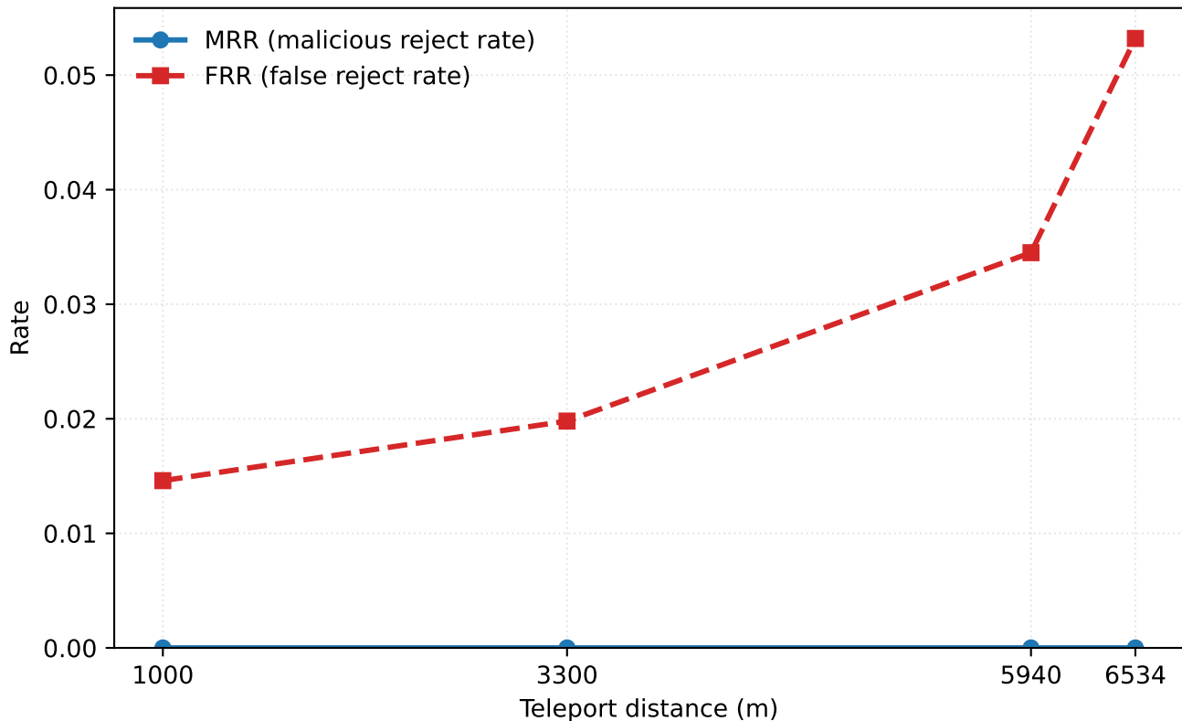
Boundary Attack Curves (T-Drive, 30 rounds)
