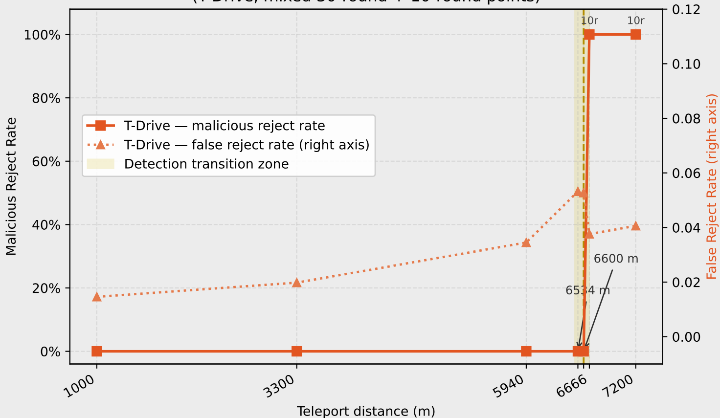
TSIP Boundary Detection: S-Curve (T-Drive, mixed 30-round + 10-round points)
