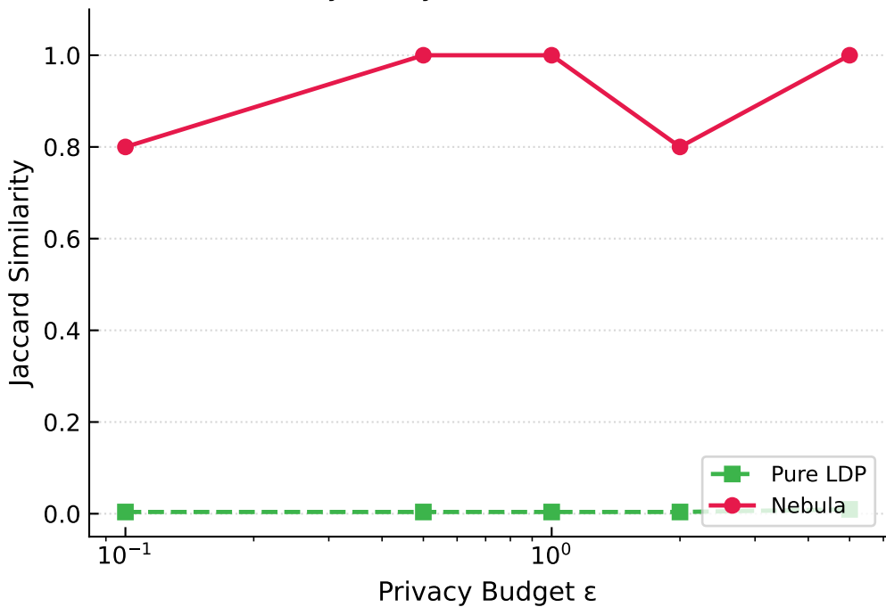
Privacy-Utility Tradeoff (mal=10%)
