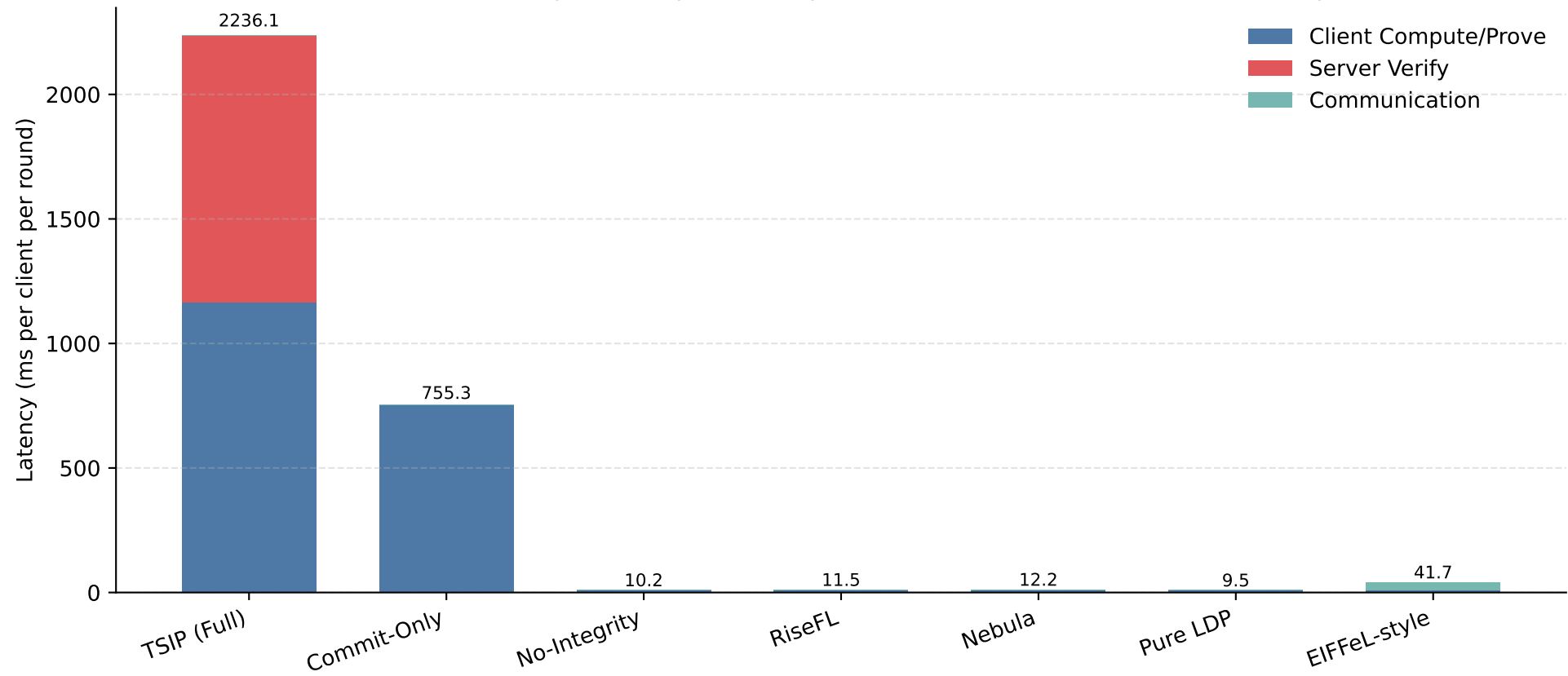
Overhead Decomposition (prover=rapidsnark, comm=baseline, link=10 Mbps)
