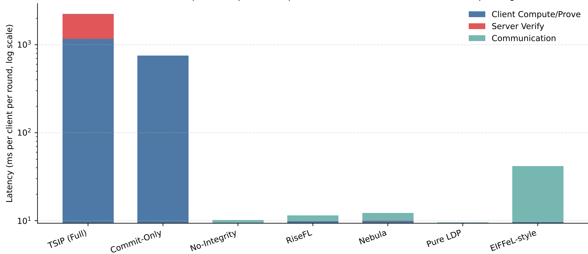
Overhead Decomposition (prover=rapidsnark, comm=baseline, link=10 Mbps) [log]
