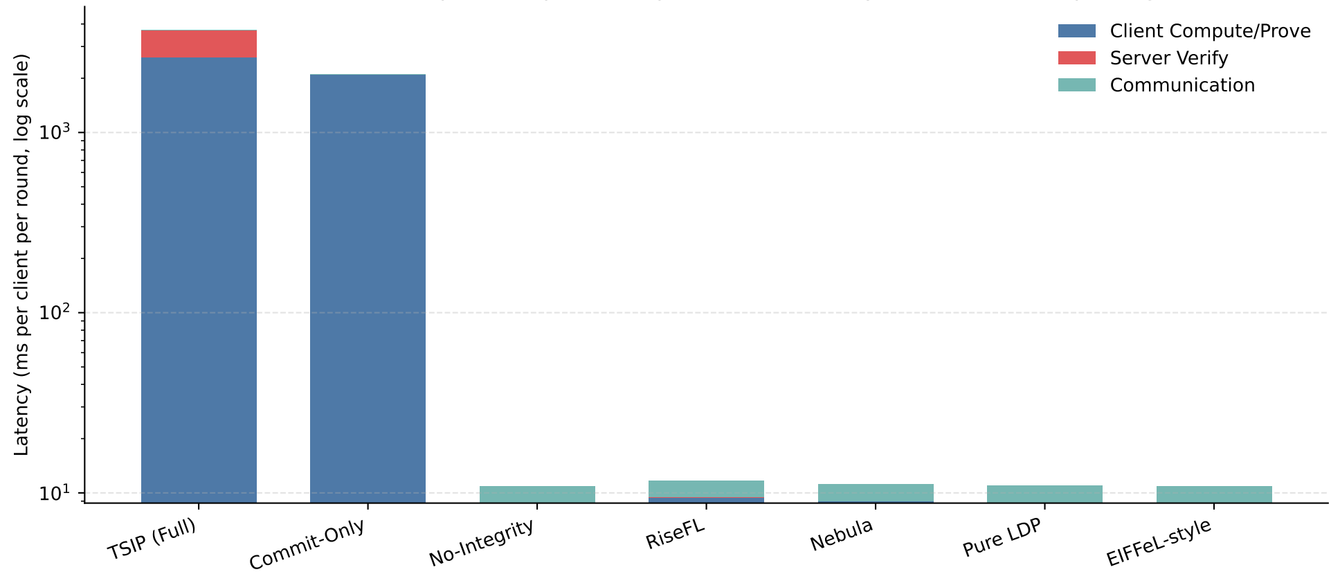
Overhead Decomposition (prover=rapidsnark, comm=system, link=10 Mbps) [log]
