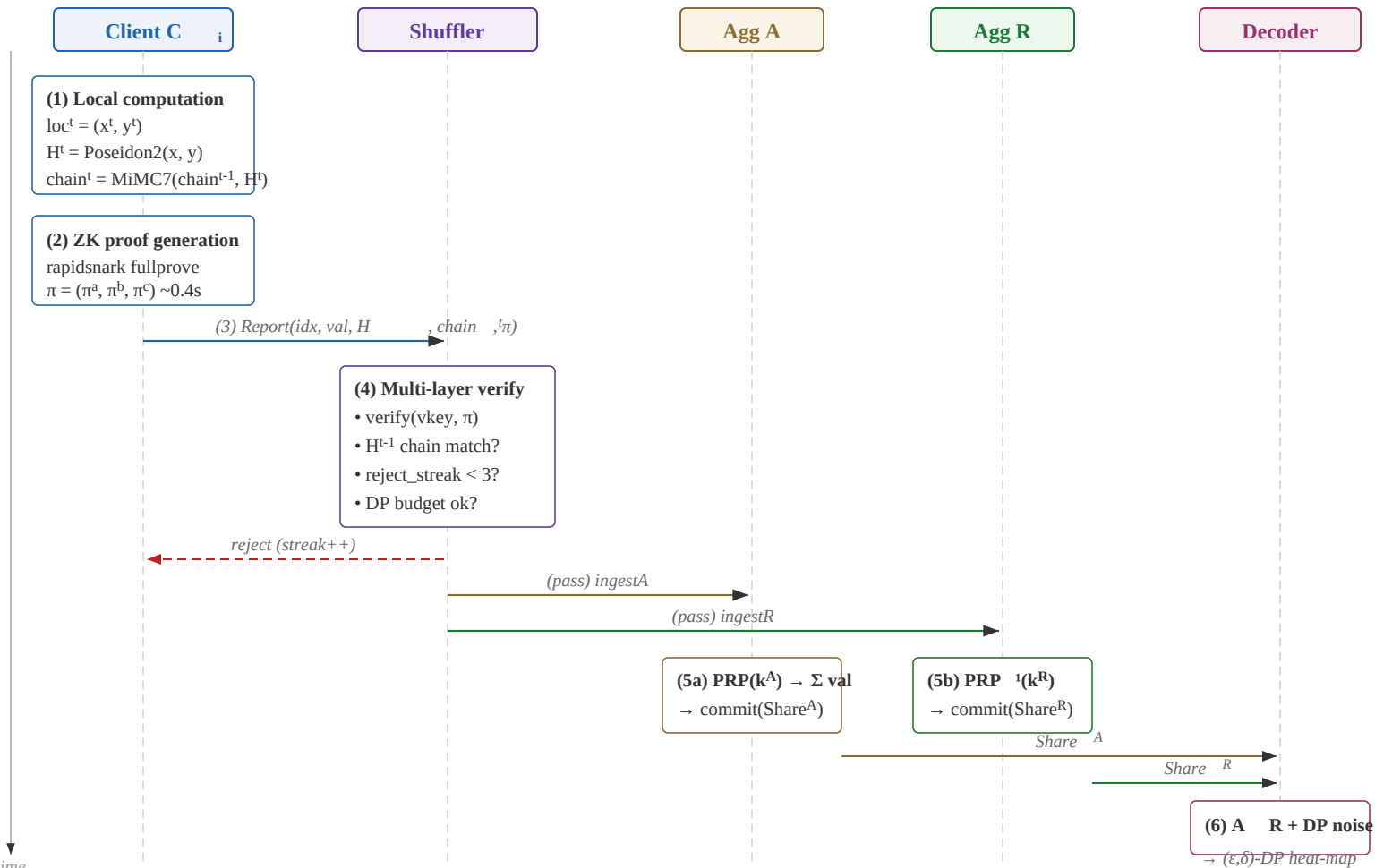
Fig. 2. TSIP Protocol Sequence (Round t \geq 1 )
