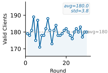
(a) Valid Clients
