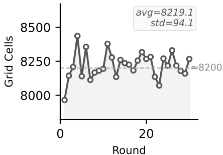
(b) Final Cells (after secure recon.)
