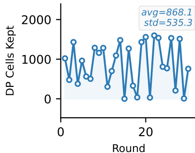
(c) DP-Filtered Cells (post-processing)
