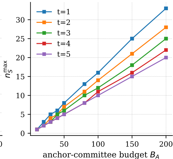
(b) tier=vehicle: effect of threshold t
