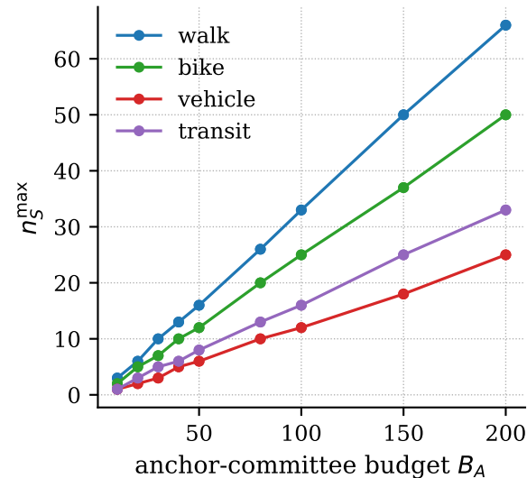
(a) t = 3 : tier-stratified bound
