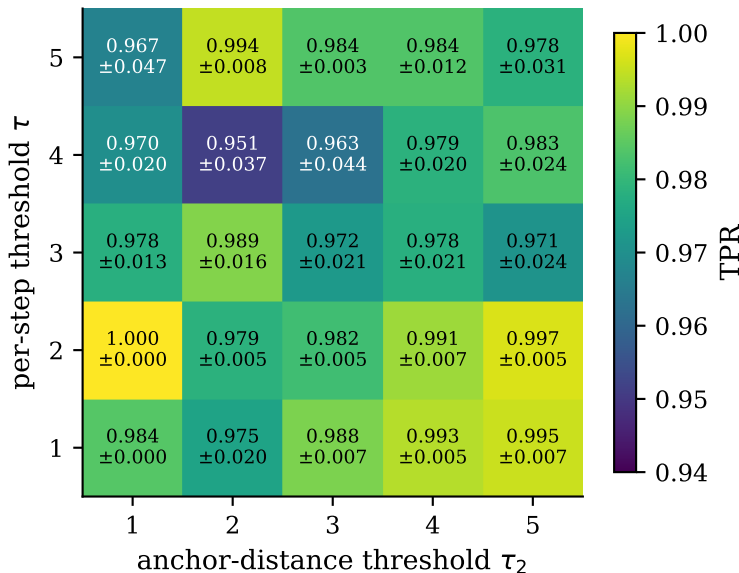
TPR on gradual-drift attack (3 seeds, mean \pm std)
