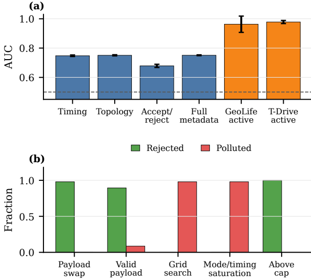
Fig. 4. Dense evaluation summary. Panel (a) reports metadata-only inference from Shuffler-visible L_S , with the dashed line marking random AUC. Panel (b) reports adaptive boundary outcomes and separates rejected attempts from accepted polluted outcomes.
