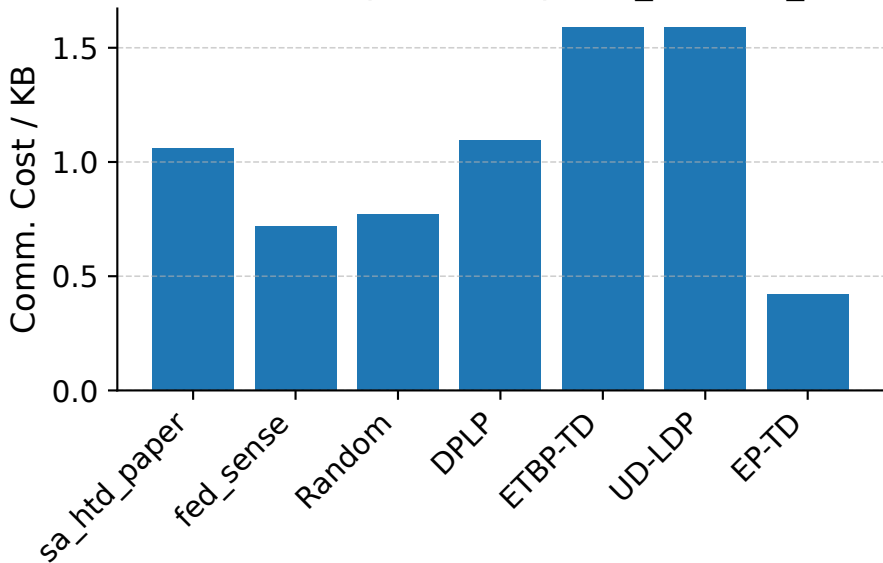
Comm. Cost Comparison (eps0.5_rho0.25_mal0.3)
