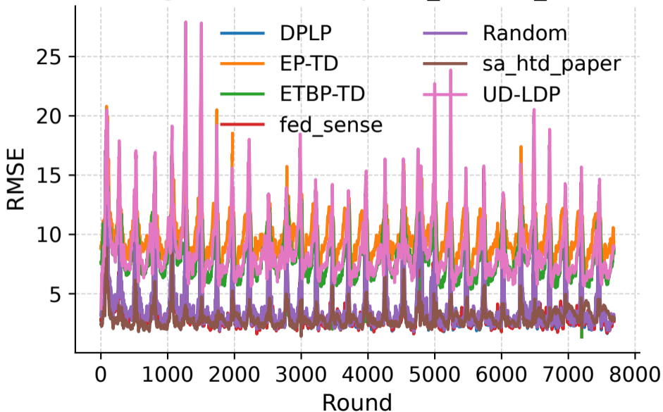
Convergence Curves (eps2.0_rho0.15_mal0.0)
