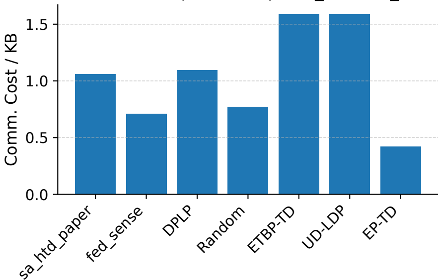
Comm. Cost Comparison (eps1.0_rho0.15_mal0.0)
