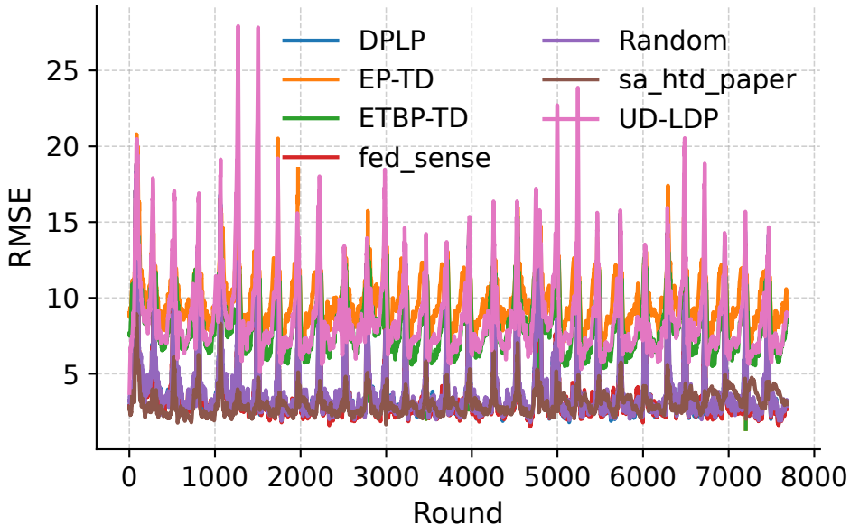
Convergence Curves (eps1.0_rho0.2_mal0.1)
