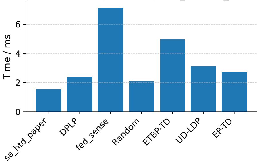
Comm. Cost Comparison (eps2.0_rho0.15_mal0.0)
