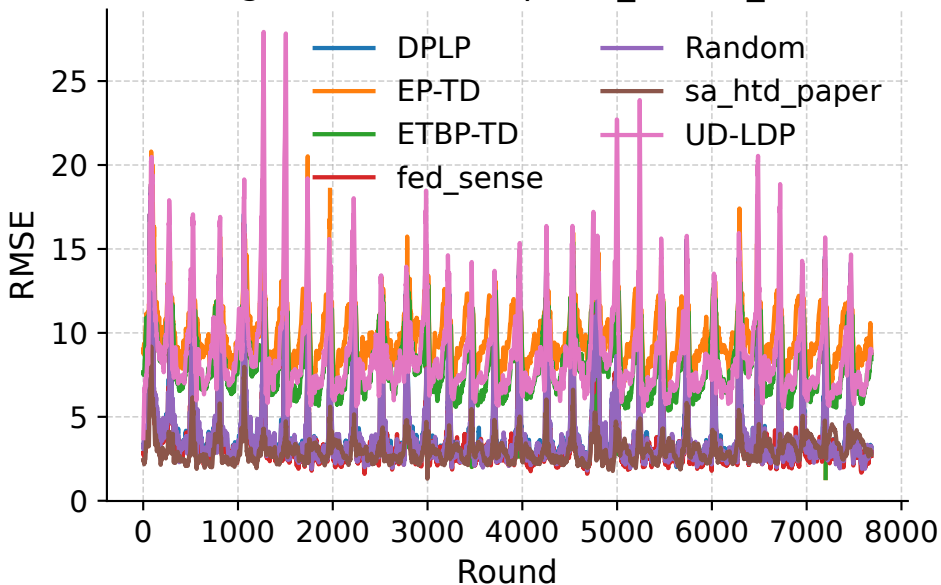
Convergence Curves (eps0.5_rho0.2_mal0.1)
