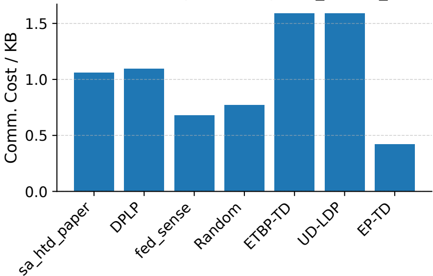
Comm. Cost Comparison (eps2.0_rho0.2_mal0.1)
