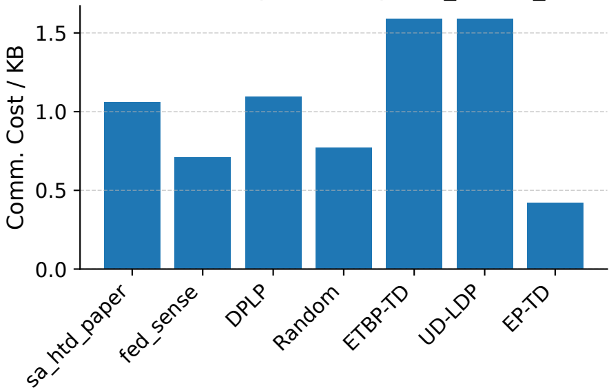
Comm. Cost Comparison (eps1.0_rho0.2_mal0.1)
