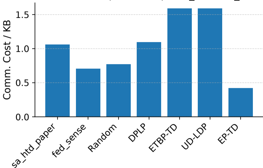
Comm. Cost Comparison (eps0.5_rho0.15_mal0.0)
