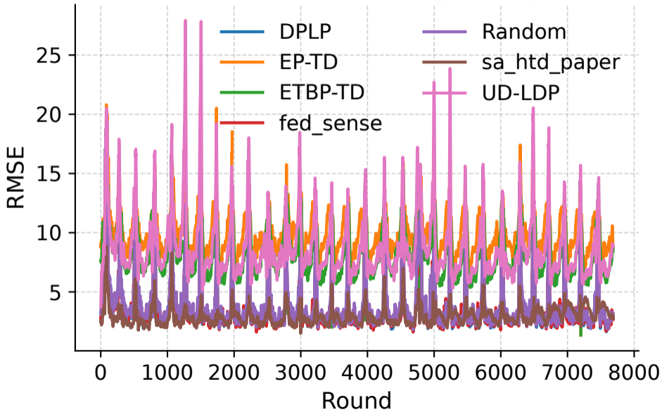
Convergence Curves (eps4.0_rho0.2_mal0.1)
