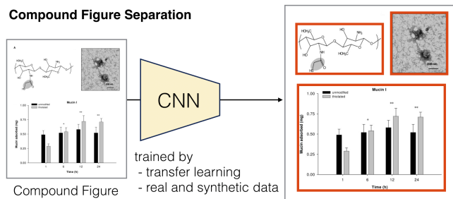
Fig. 1. We propose a new approach for segmenting a compound figure into its component subfigures. We take a data driven approach using CNNs, with transfer learning and exemplar synthesis to overcome limited training datasets.
