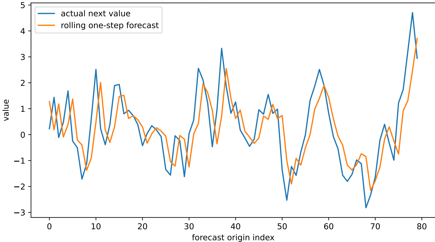
Rolling one-step forecasts; RMSE = 0.953
