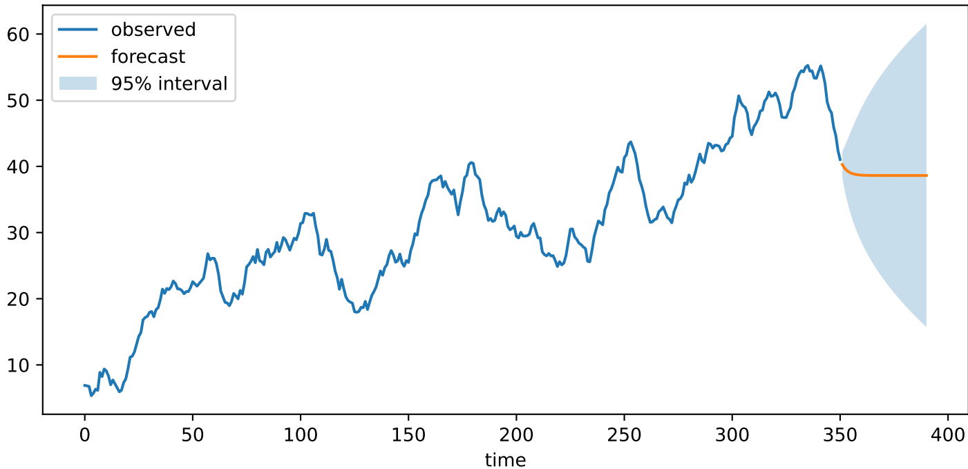
Forecast from ARIMA(1, 1, 1)
