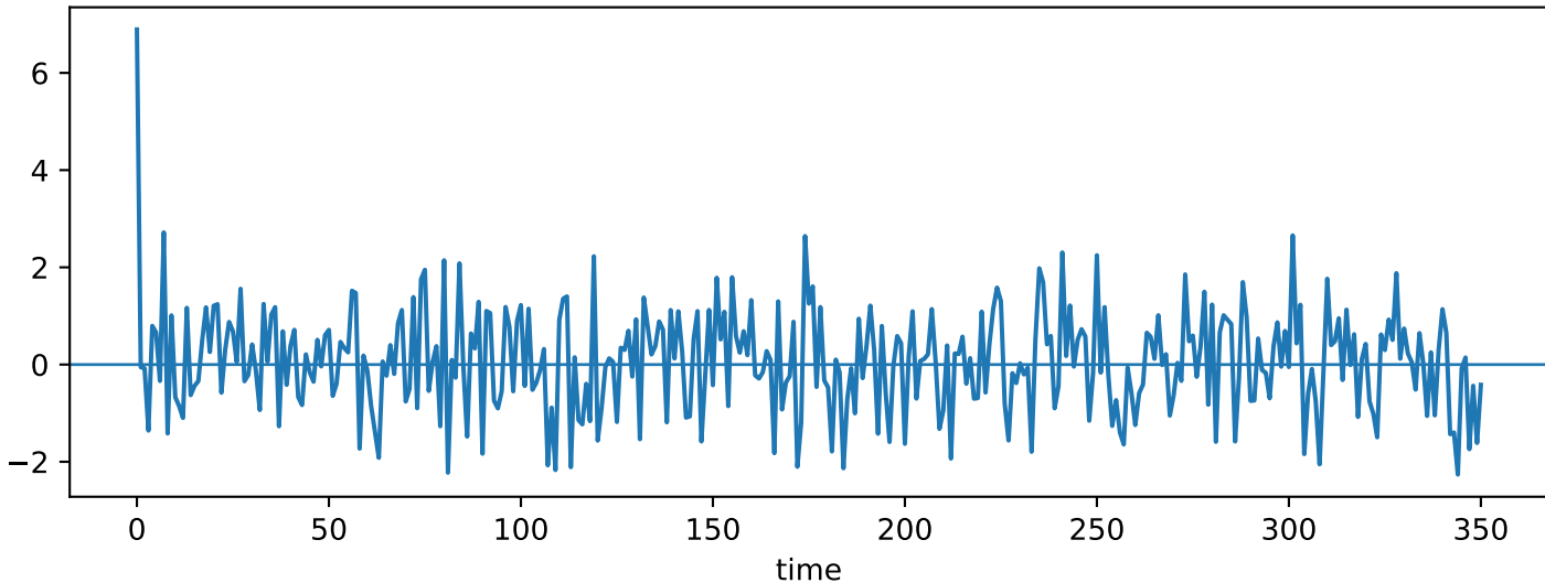
ARIMA residuals
