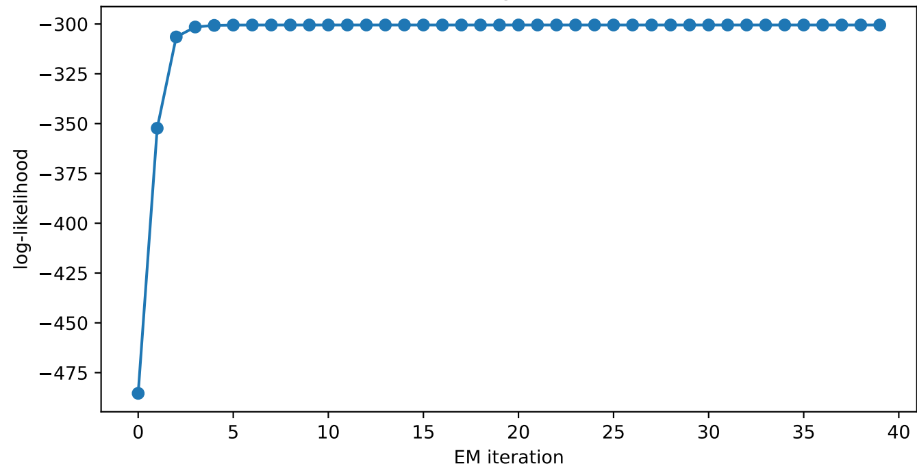
Baum--Welch log-likelihood trace
