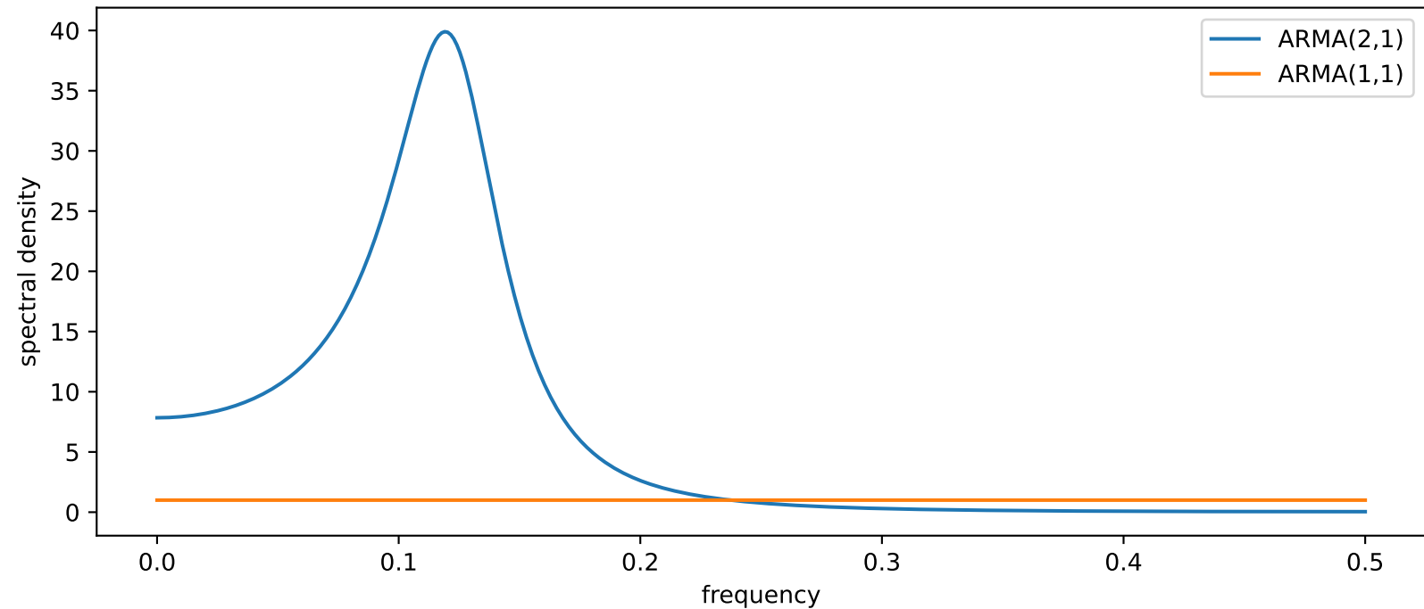
ARMA spectra from polynomial ratios
