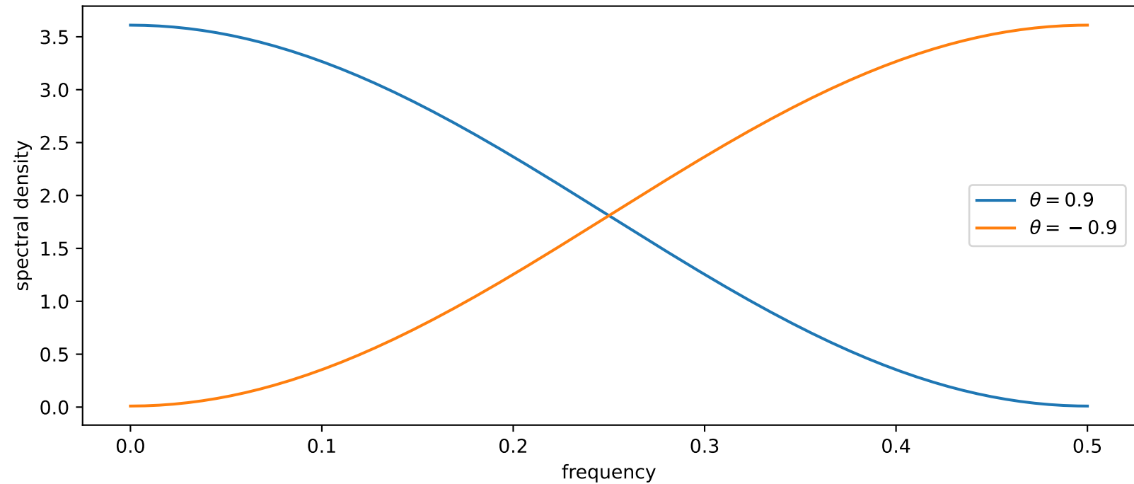
MA(1) spectra
