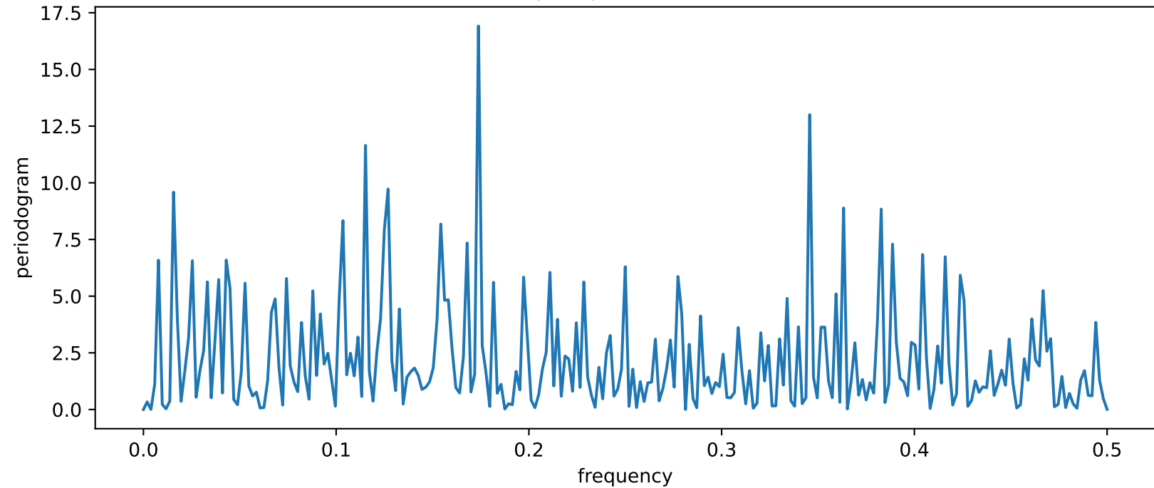
A finite-sample spectrum of white noise
