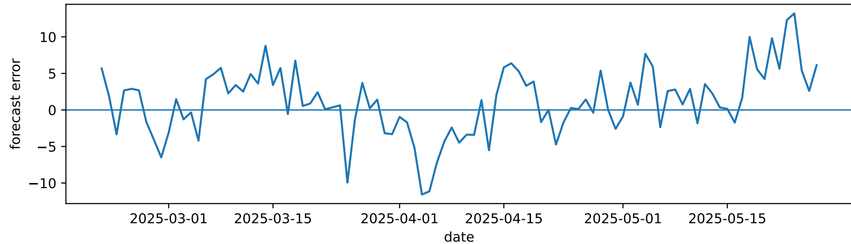
Test errors for ridge
