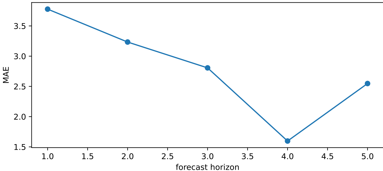
Rolling-origin MAE by horizon
