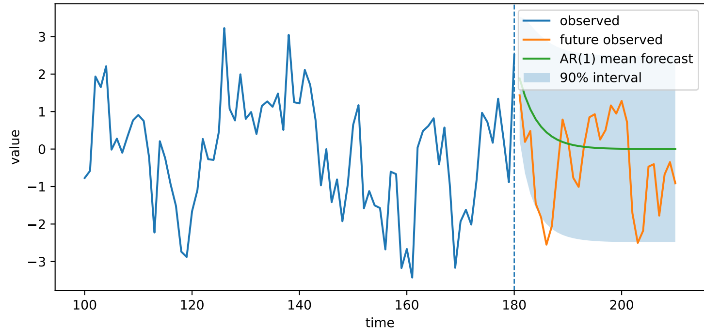
Model-based AR(1) prediction interval
