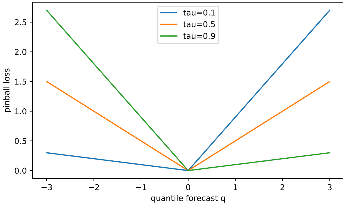
Pinball loss for one observed value
