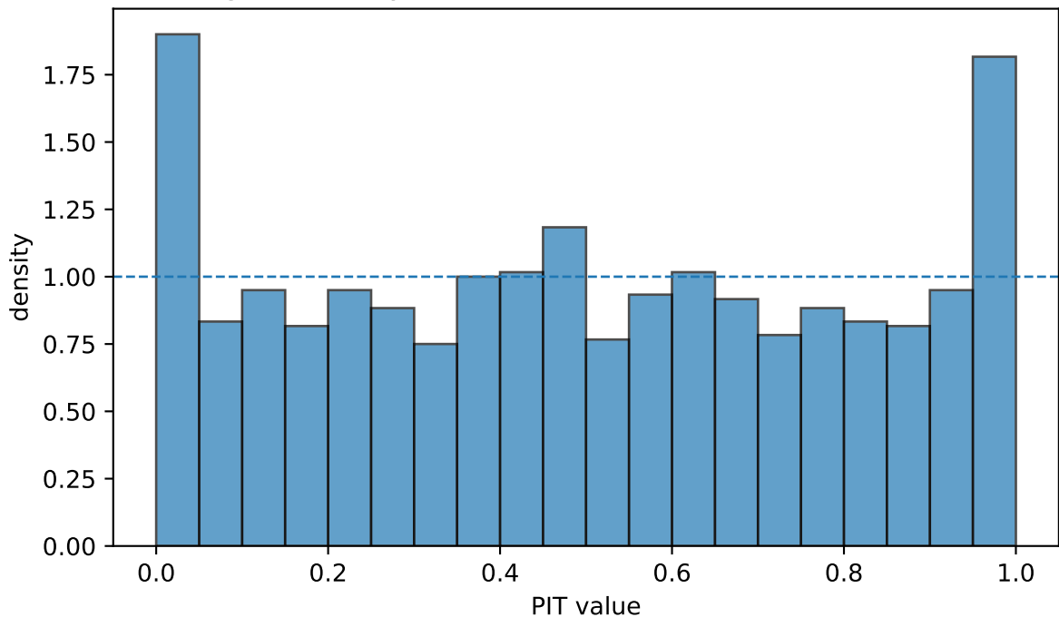
PIT histogram: heavy-tailed observations under Gaussian forecasts
