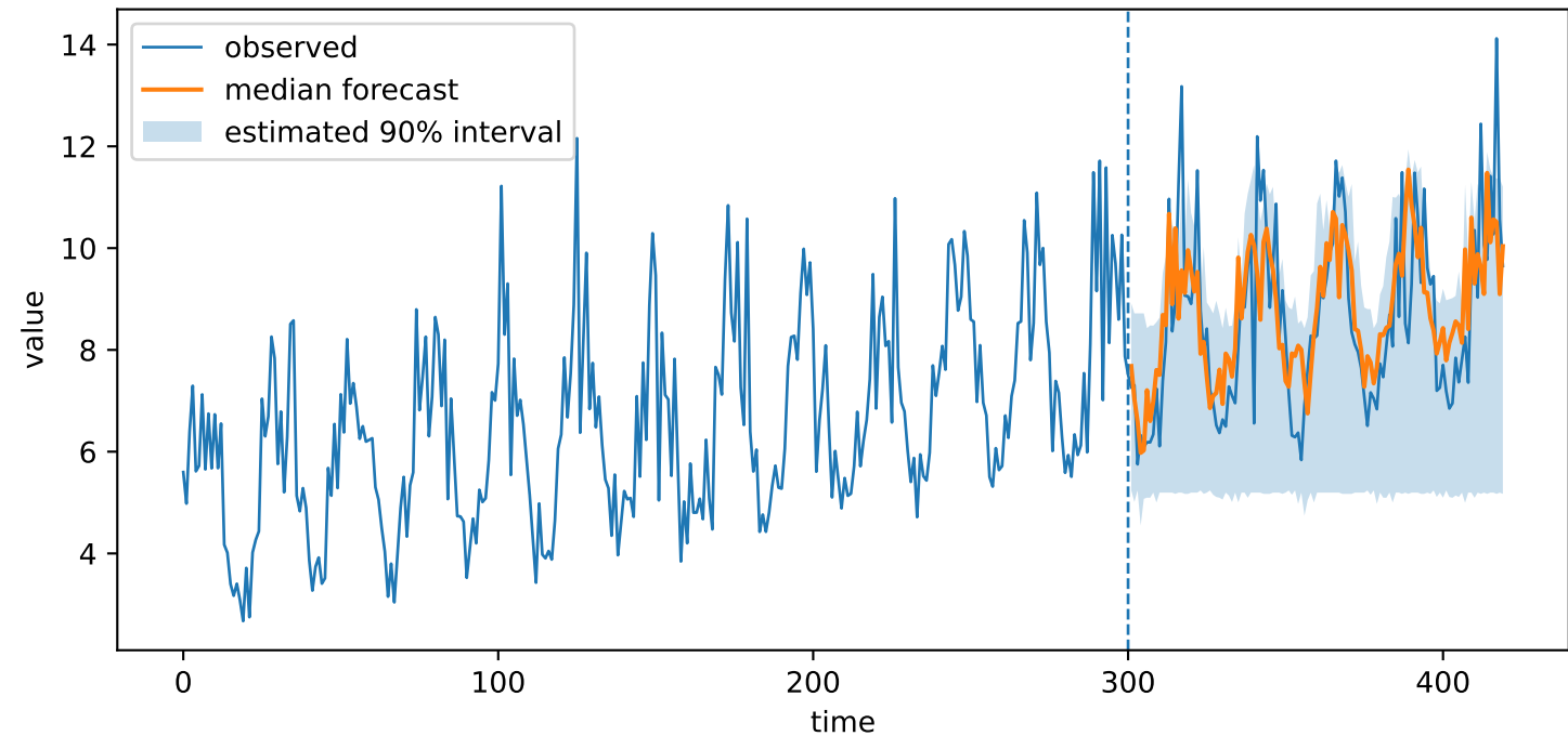
Quantile-regression forecast interval
