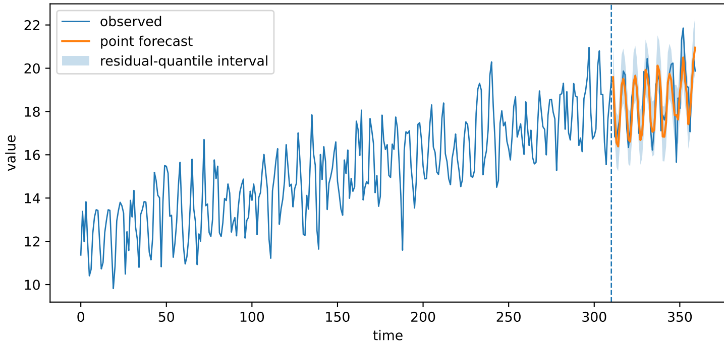
Residual-bootstrap style interval
