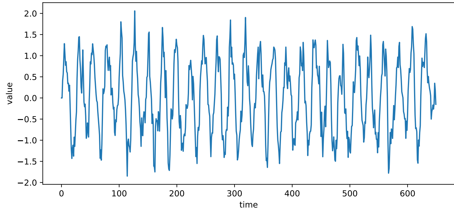
Synthetic nonlinear seasonal time series
