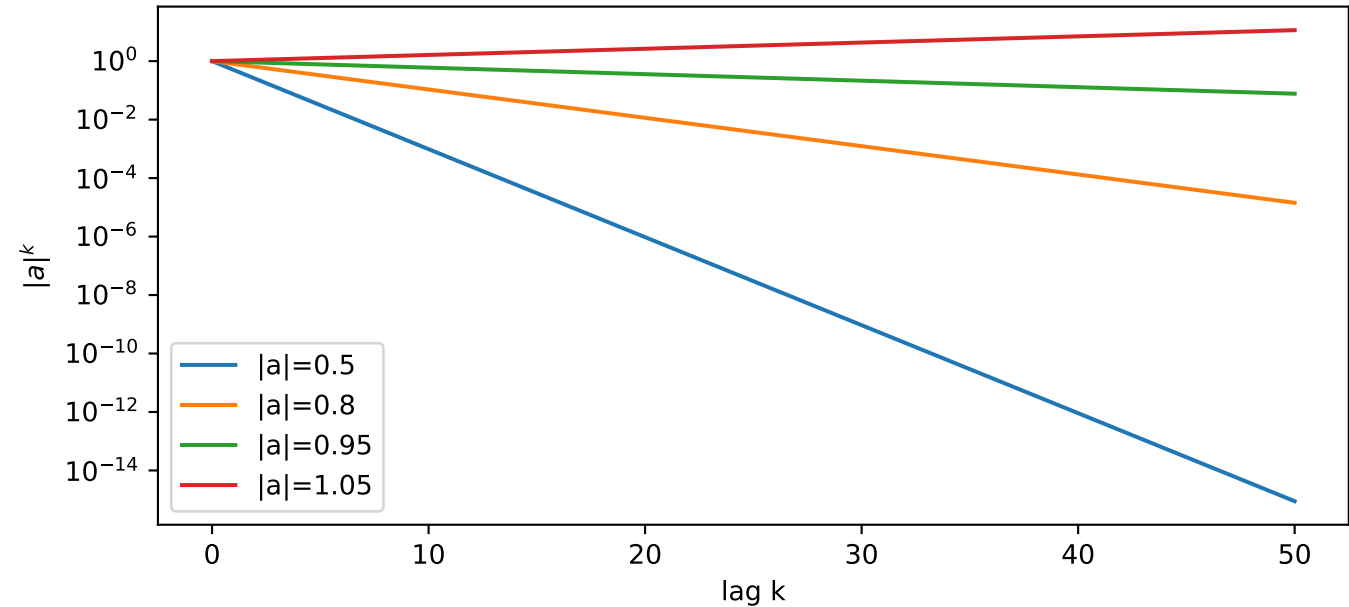
Vanishing and exploding gradient intuition
