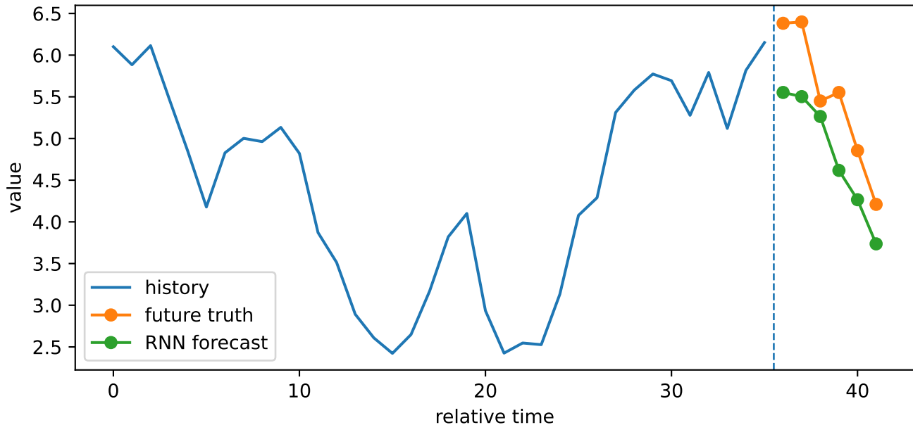
Direct multi-horizon RNN forecast
