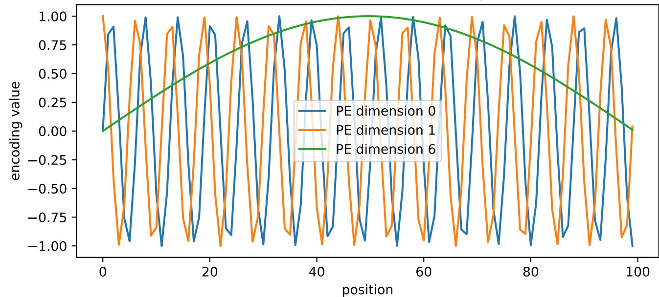
Sinusoidal positional encoding
