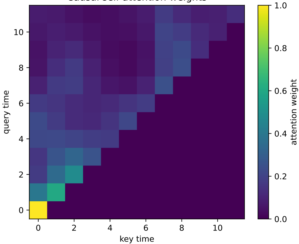
Causal self-attention weights
