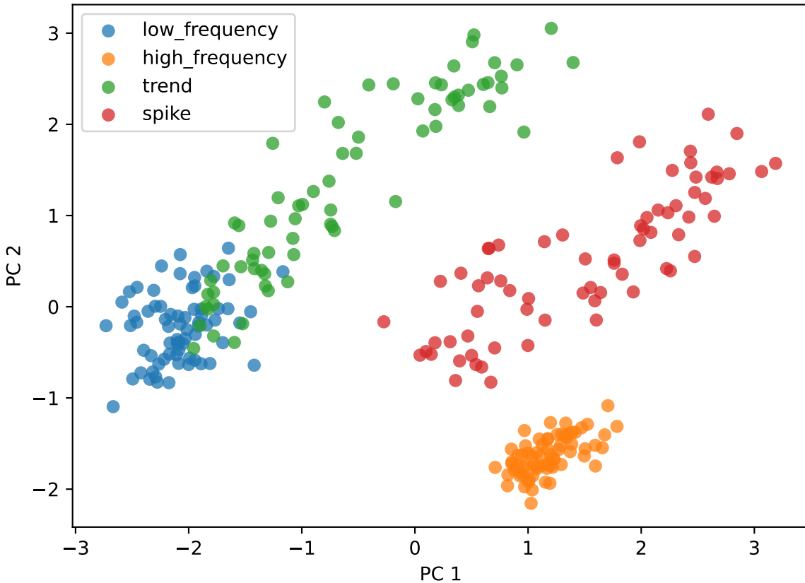
Feature-based representation of time-series windows
