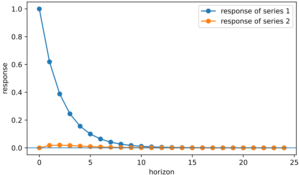
Estimated impulse response to a shock in series 1
