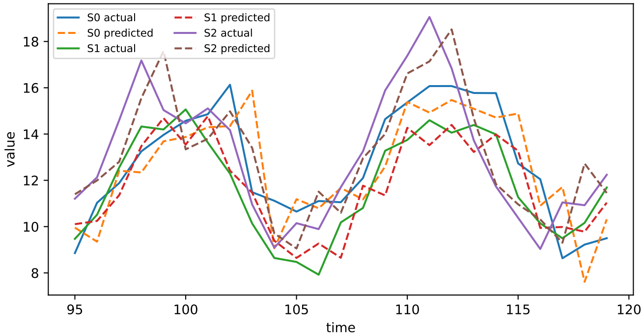
Pooled lag model on panel data
