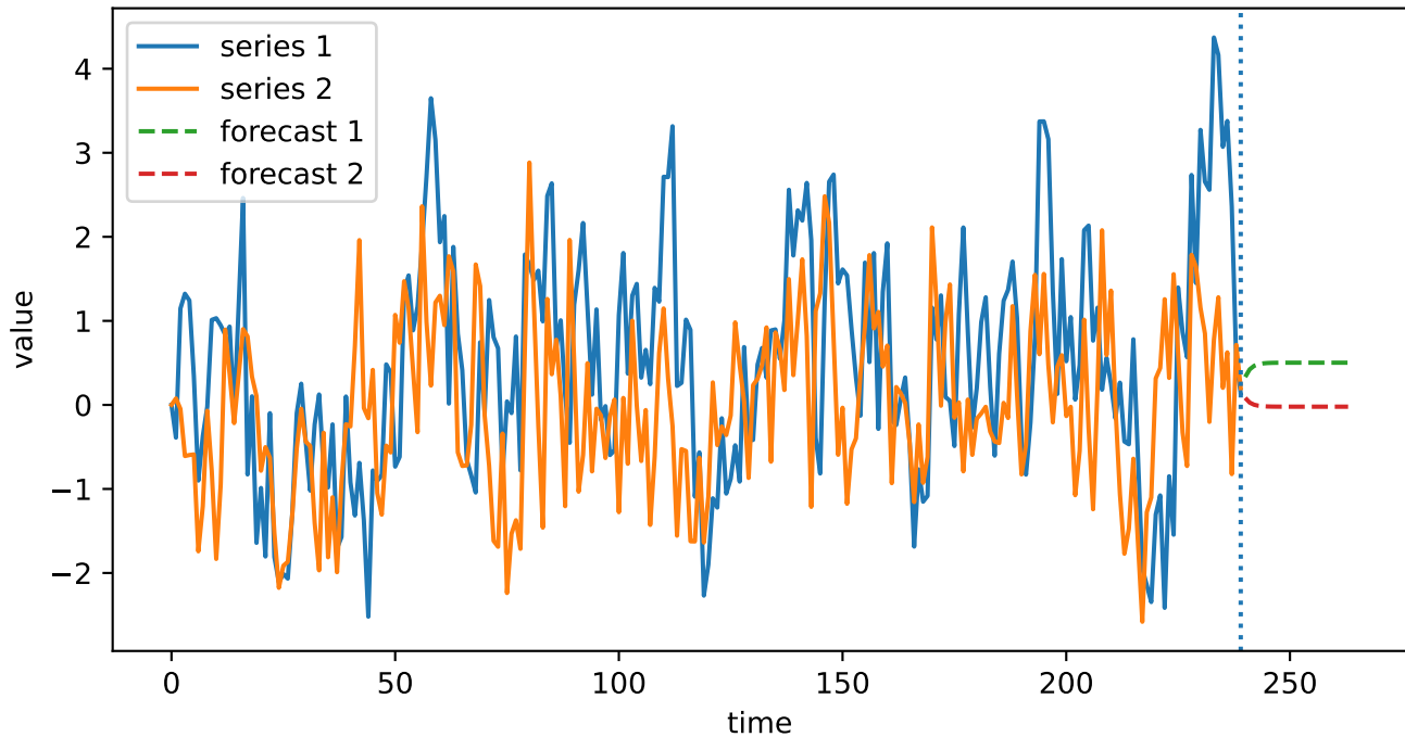
VAR(1) simulation and recursive forecast
