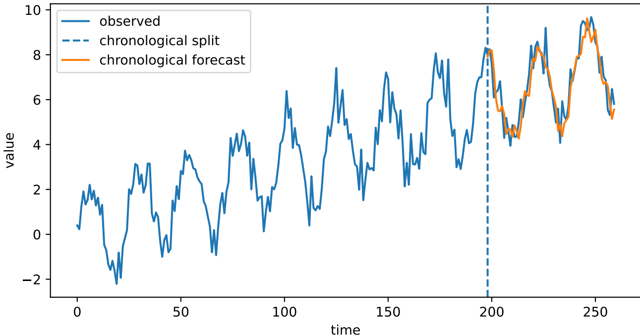
Chronological evaluation: forecasting the future block
