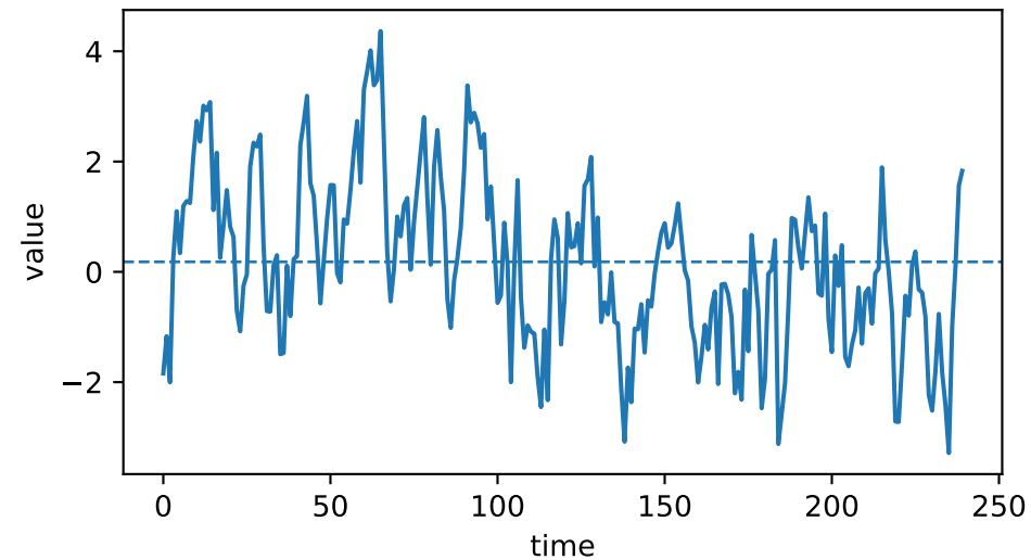
AR(1), \phi=0.7
