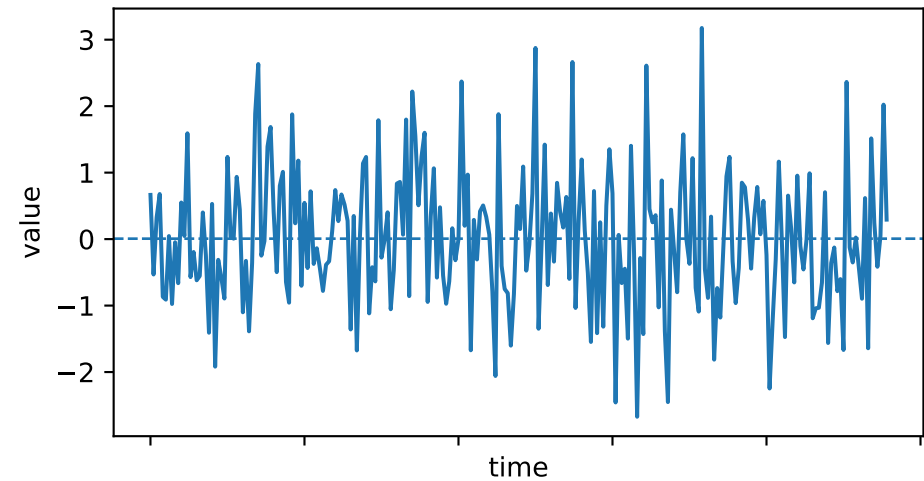
AR(1), \phi=0.7
