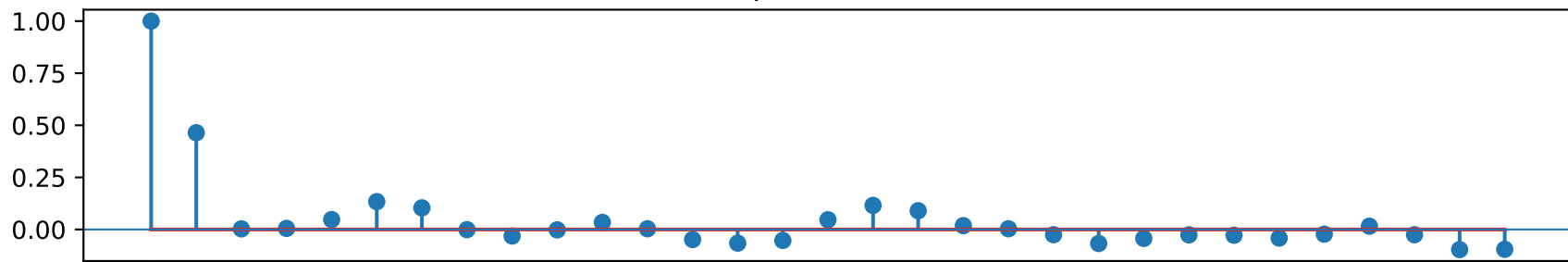
Sample ACF: MA(1)
