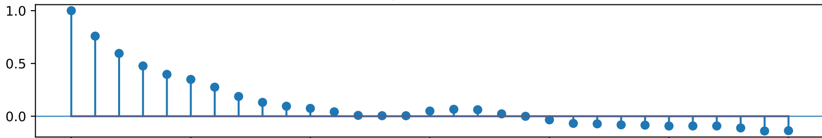
Sample ACF: AR(1)
