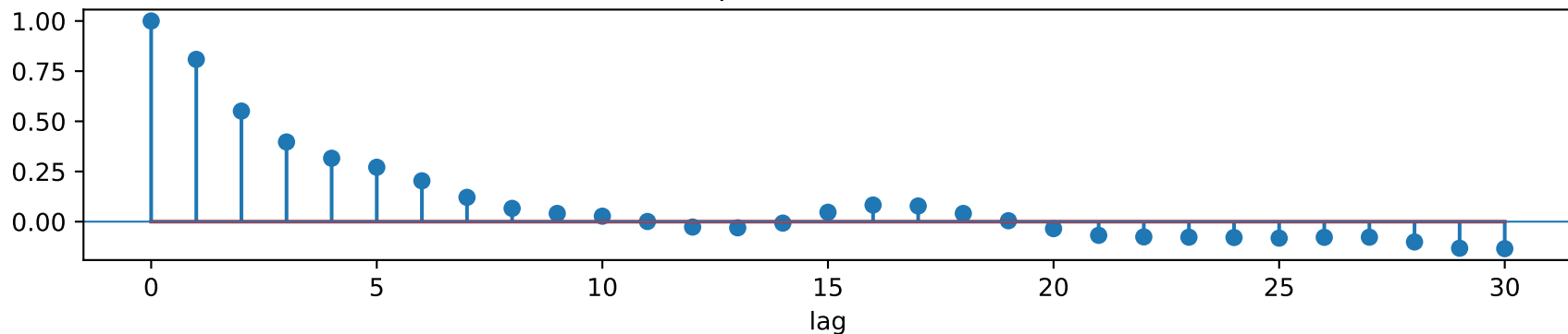
Sample ACF: ARMA(1,1)
